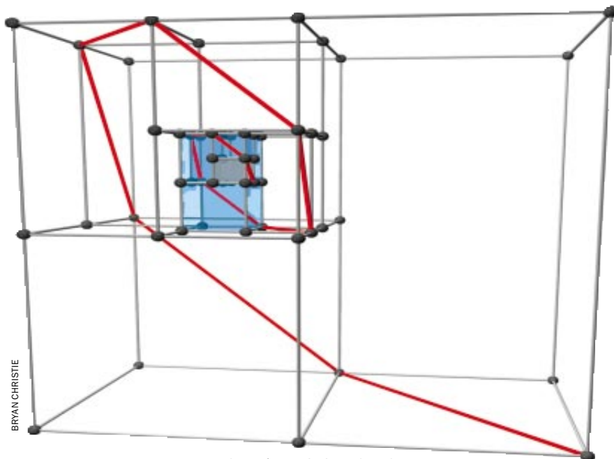
SPIRALING CUBOIDS also form Padovan numbers.
